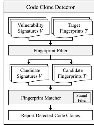
Fig. 7: Overview of the Code Clone Detector
