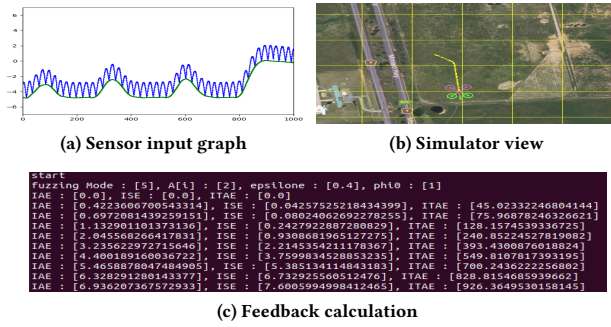
Figure 2: Screenshot of a SENSORFUZZ demonstration.
