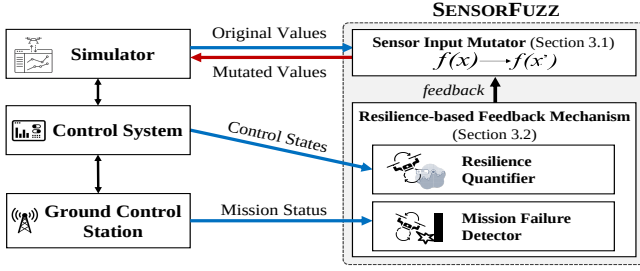
Figure 1: Architecture of SENSORFUZZ.
