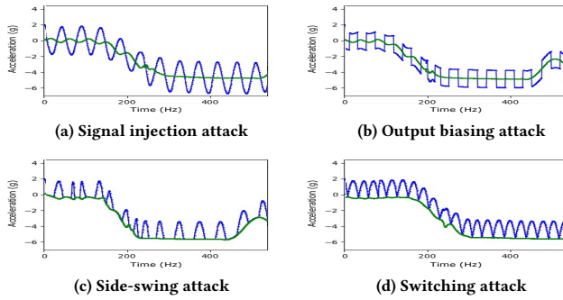
Figure 3: Existing sensor attacks [7–11] detected by SENSORFUZZ.
