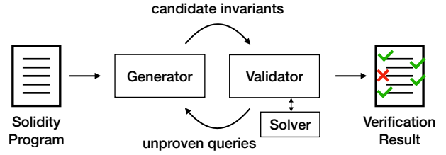
Fig. 5. Algorithm overview.
